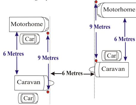
Hardstanding Layout Nose To Tail
